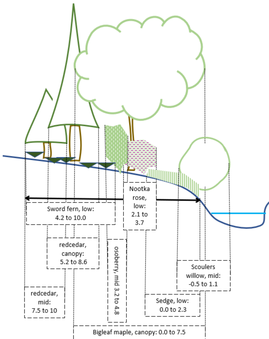
Figure 1: Sketch of line-intercept transect method for riparian/floodplain vegetation. Plants encountered along the transect are recorded by species and height class, with the start and end locations of their cover presence (in m) directly above or below the transect tape. Note that plant species occurrences within the same height class are combined if no gaps in cover greater than 0.15 m occur. In the sketch, Scoulers willow overhangs within 1 m of the bankfull elevation and the overhang distance is recorded as a negative value. No overhang distance is recorded for bigleaf maple, as it is not within 1 m elevation of bankfull.
